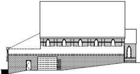
WEST ELEVATION
